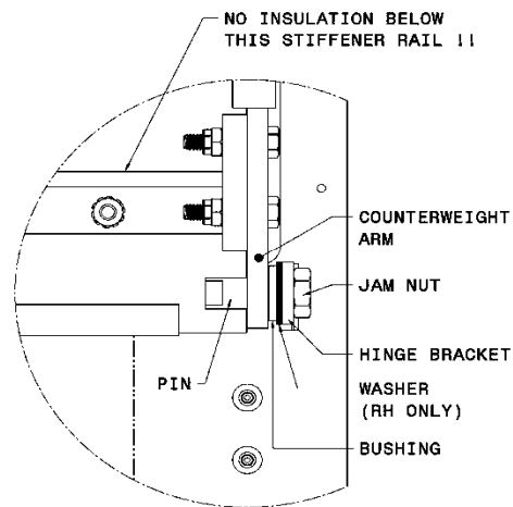
RH HINGE DETAIL
